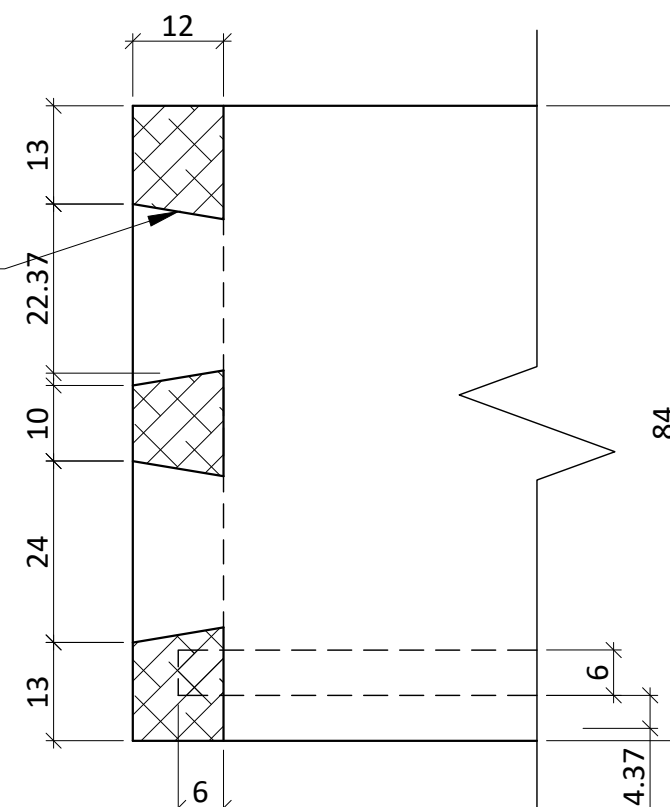
POST SECONDARY DRAWER CORNER JOINERY SCALE 1 : 1 DOVE TAIL FRONT ONLY & RABBET BACK
