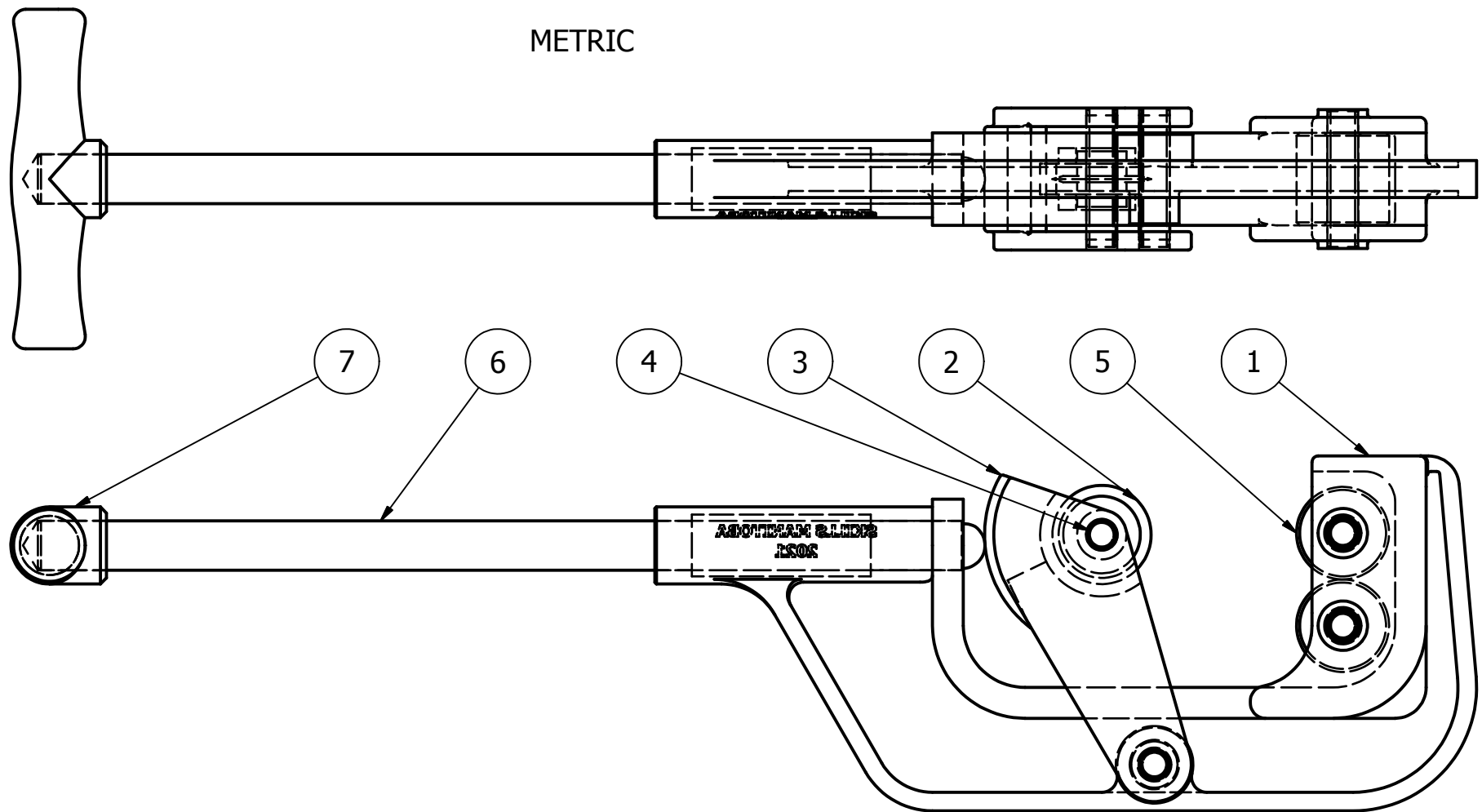
GENERAL LAYOUT ( 1 : 2 )
